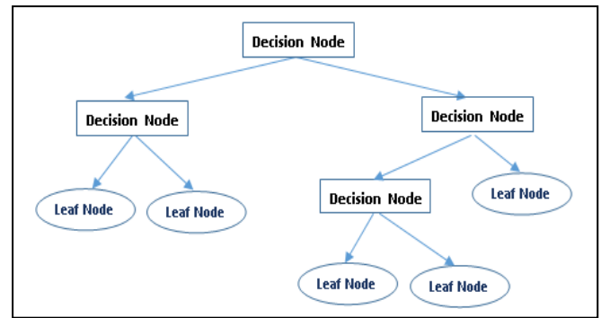
Figure 2. Decision Trees Model
