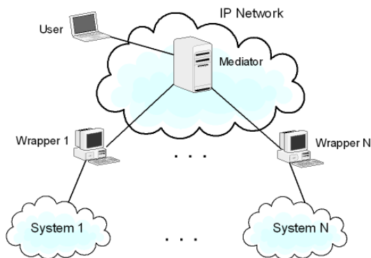
Figure 4. SeNsIM architecture
